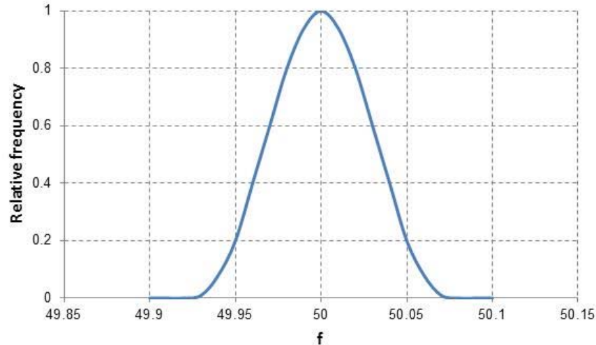
Figure 12. Relative frequency of 50 Hz network frequency
