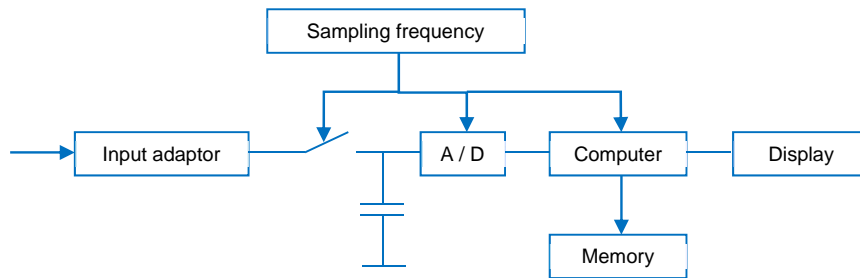
Figure 10. General block-structure of digital measurement systems
