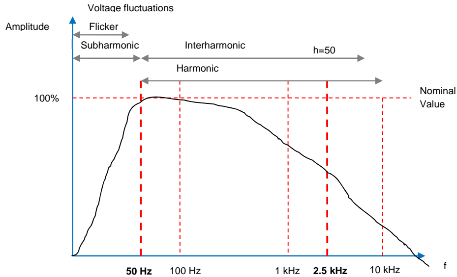
Figure 1. Frequency range of disruptions
