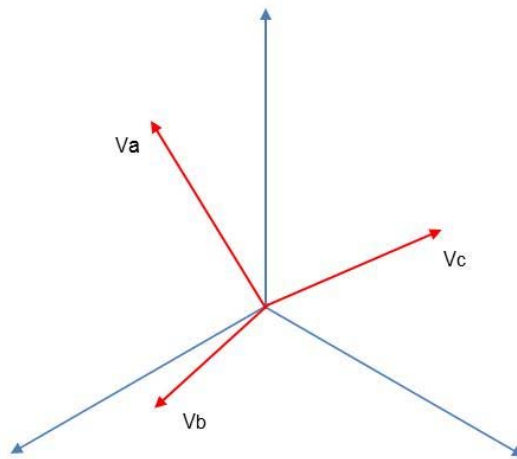
Figure 7. Voltage unbalance
