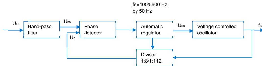
Figure 11. Phase-locked-loop element (PLL)
