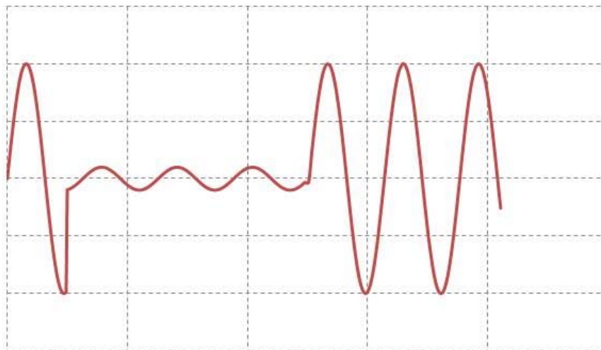
Figure 5. Voltage dip
