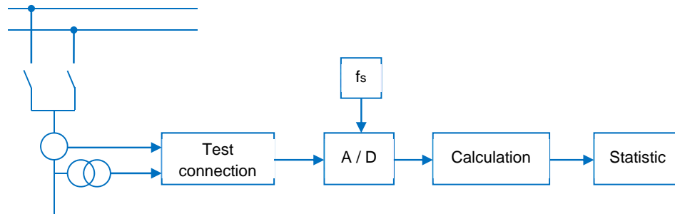
Figure 19. Overall arrangement of a recording line
